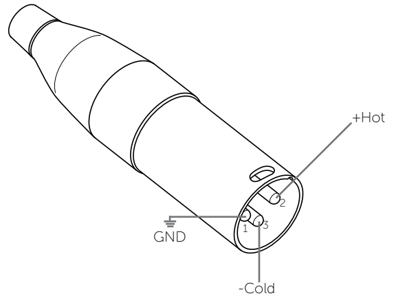
Figure 4.2: XLR-M diagram
